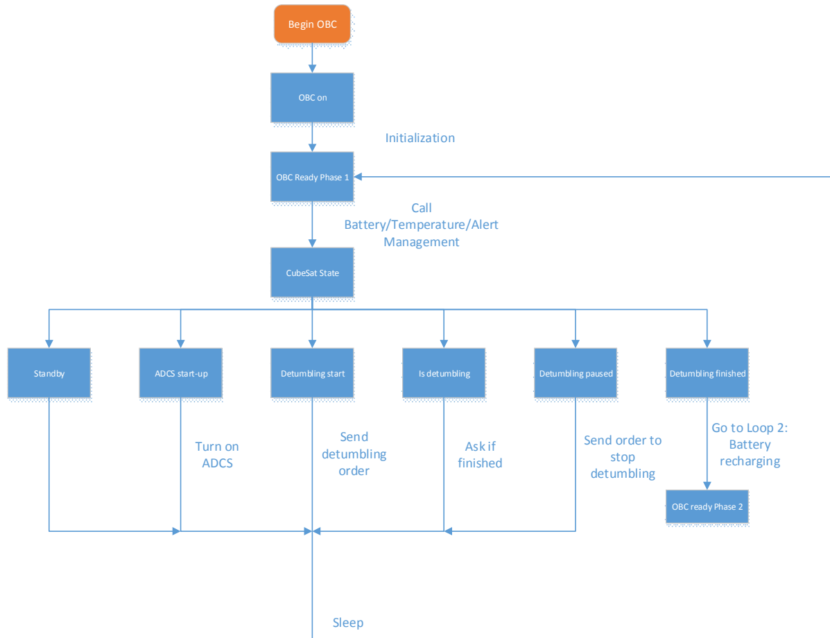
Algorithm for OBC loop 1: detumbling
